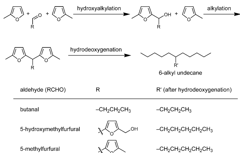
Scheme 2. Formation of 1,1-bisylvylalkanes by hydroxyalkylation/alkylation from 2MF and an aldehyde with subsequent hydrodeoxygenation to 6-alkyl undecane.
